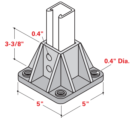
CS-PB-20S (1-5/8" x 1-5/8"), CS-PB-10S (1-1/8" x 1-1/2")
